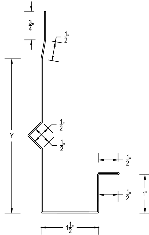
J-FASCIA WITH STIFFENER & RETURN _____ LINEAR FEET (120" PCS)
