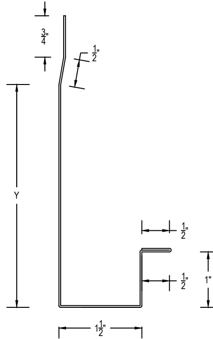
J-FASCIA WITH RETURN LINEAR FEET (120" PCS)
