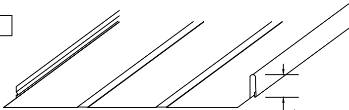
1-1/2" SNAP SEAM PANEL WITH 2 LOW FLAT BEADS 11-3/4", 15-3/4", 17-3/4", AND 19-3/4" WIDE PANEL PRE-NOTCHED & PRE-TABBED
