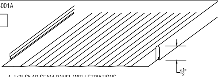
1-1/2" SNAP SEAM PANEL WITH STRIATIONS 11-3/4", 15-3/4", 17-3/4", AND 19-3/4" WIDE PANEL PRE-NOTCHED & PRE-TABBED
