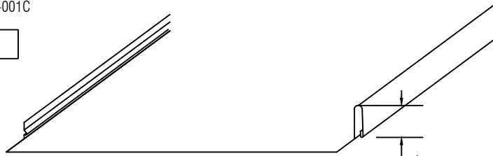
1-1/2" SNAP SEAM PANEL, SMOOTH 11-3/4", 15-3/4", 17-3/4", AND 19-3/4" WIDE PANEL PRE-NOTCHED & PRE-TABBED
