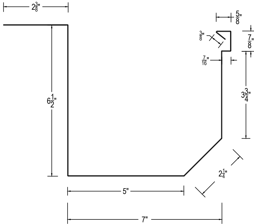
SEAMLESS GUTTER PROFILE
