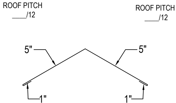
STANDING SEAM RIDGE CAP-SMALL _____ LINEAR FEET (120" PCS)
