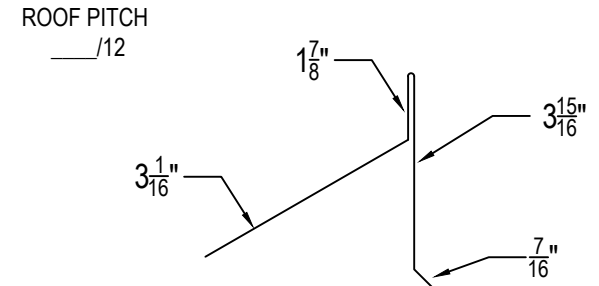
STANDING SEAM VERTICAL RIDGE CLEAT _____ LINEAR FEET (120" PCS)
