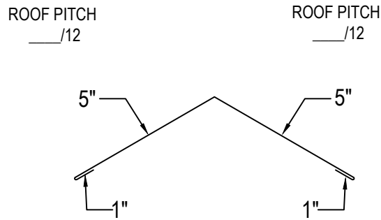
STANDING SEAM HIP CAP-SMALL _____ LINEAR FEET (120" PCS)
