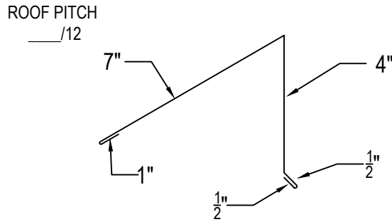
STANDING SEAM VERTICAL RIDGE _____ LINEAR FEET (120" PCS)
