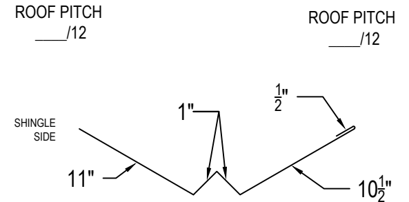
SHINGLE TO STANDING SEAM VALLEY _____ LINEAR FEET (120" PCS)
