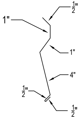
STANDING SEAM SURFACE MOUNT REGLET ____ LINEAR FEET (120" PCS)
