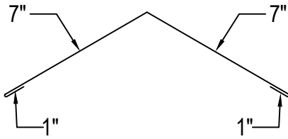
STANDING SEAM RIDGE CAP-LARGE ____ LINEAR FEET (120" PCS)
