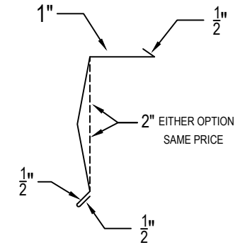
STANDING SEAM SAW CUT REGLET ____ LINEAR FEET (120" PCS)
