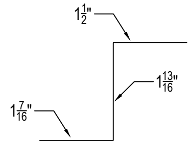
STANDING SEAM SAW CUT REGLET ____ LINEAR FEET (120" PCS)
