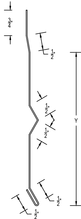
FASCIA TYPE 2 LINEAR FEET (120" PCS)
