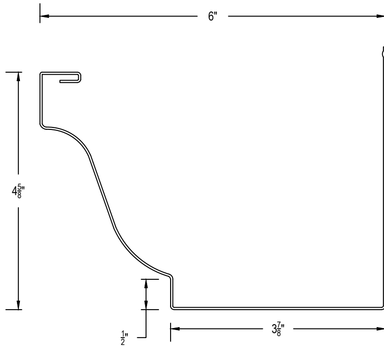
SEAMLESS GUTTER PROFILE
