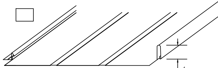
1-1/2" NAIL LEG PANEL WITH 2 LOW FLAT BEADS 10-3/4", 14-3/4", AND 18-3/4" WIDE PANEL PRE-NOTCHED & PRE-TABBED
