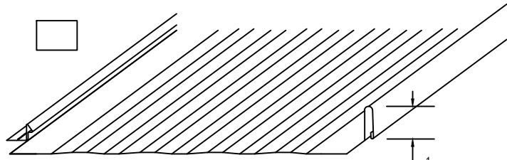
1-1/2" NAIL LEG PANEL WITH STRIATIONS 10-3/4", 14-3/4", AND 18-3/4" WIDE PANEL PRE-NOTCHED & PRE-TABBED
