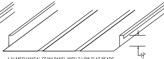
1.5" MECHANICAL SEAM PANEL WITH 2 LOW FLAT BEADS 11.75", 15.75", 17.75", AND 19.75" WIDE PANEL PRE-NOTCHED
