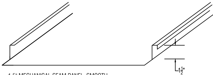
1.5" MECHANICAL SEAM PANEL, SMOOTH 11.75", 15.75", 17.75", AND 19.75" WIDE PANEL PRE-NOTCHED
