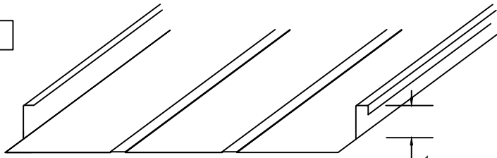
1-1/2" MECHANICAL SEAM PANEL WITH 2 LOW FLAT BEADS 11-3/4", 15-3/4", AND 19-3/4" WIDE PANEL PRE-NOTCHED
