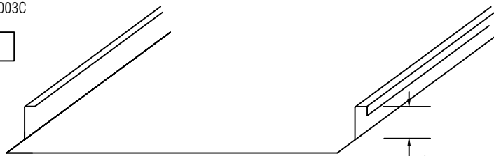
1-1/2" MECHANICAL SEAM PANEL, SMOOTH 11-3/4", 15-3/4" AND 19-3/4" WIDE PANEL PRE-NOTCHED
