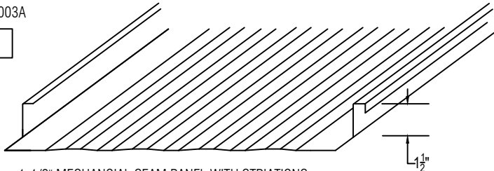
1-1/2" MECHANICAL SEAM PANEL WITH STRIATIONS 11-3/4", 15-3/4" AND 19-3/4" WIDE PANEL PRE-NOTCHED
