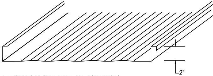
2" MECHANICAL SEAM PANEL WITH STRIATIONS 10", 12", 16", AND 18" WIDE PANEL
