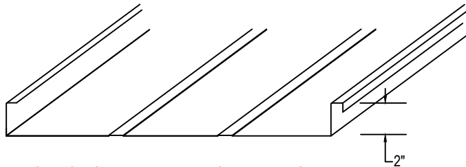
2" MECHANICAL SEAM PANEL WITH 2 LOW FLAT BEADS 10", 12", 16", AND 18" WIDE PANEL
