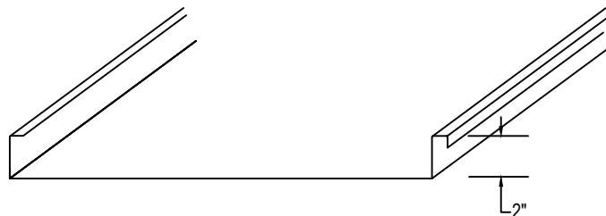
2" MECHANICAL SEAM PANEL, SMOOTH 10", 12", 16", AND 18" WIDE PANEL
