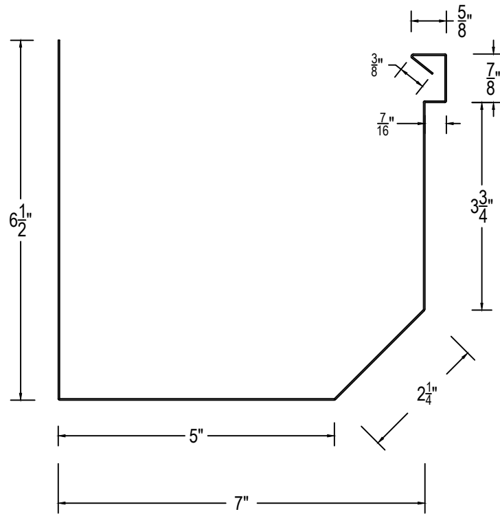
SEAMLESS GUTTER PROFILE
