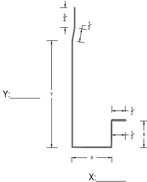
J-FASCIA WITH RETURN _____ LINEAR FEET (120" PCS)
