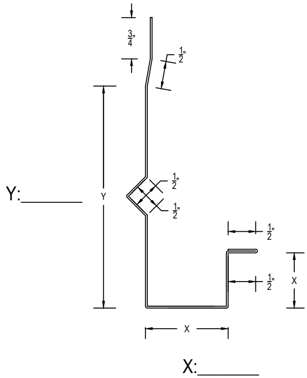
J-FASCIA WITH STIFFENER & RETURN _____ LINEAR FEET (120" PCS)
