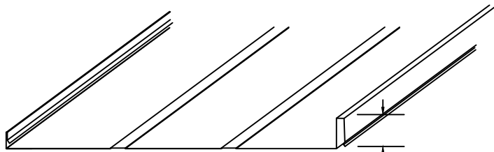
1-3/4" SNAP SEAM PANEL WITH 2 LOW FLAT BEADS 10", 12", 16", AND 18" WIDE PANEL
