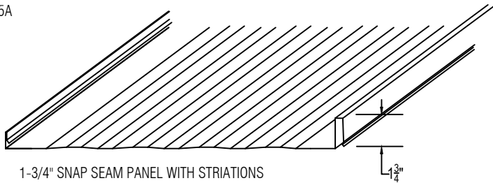
1-3/4" SNAP SEAM PANEL WITH STRIATIONS 10", 12", 16", AND 18" WIDE PANEL
